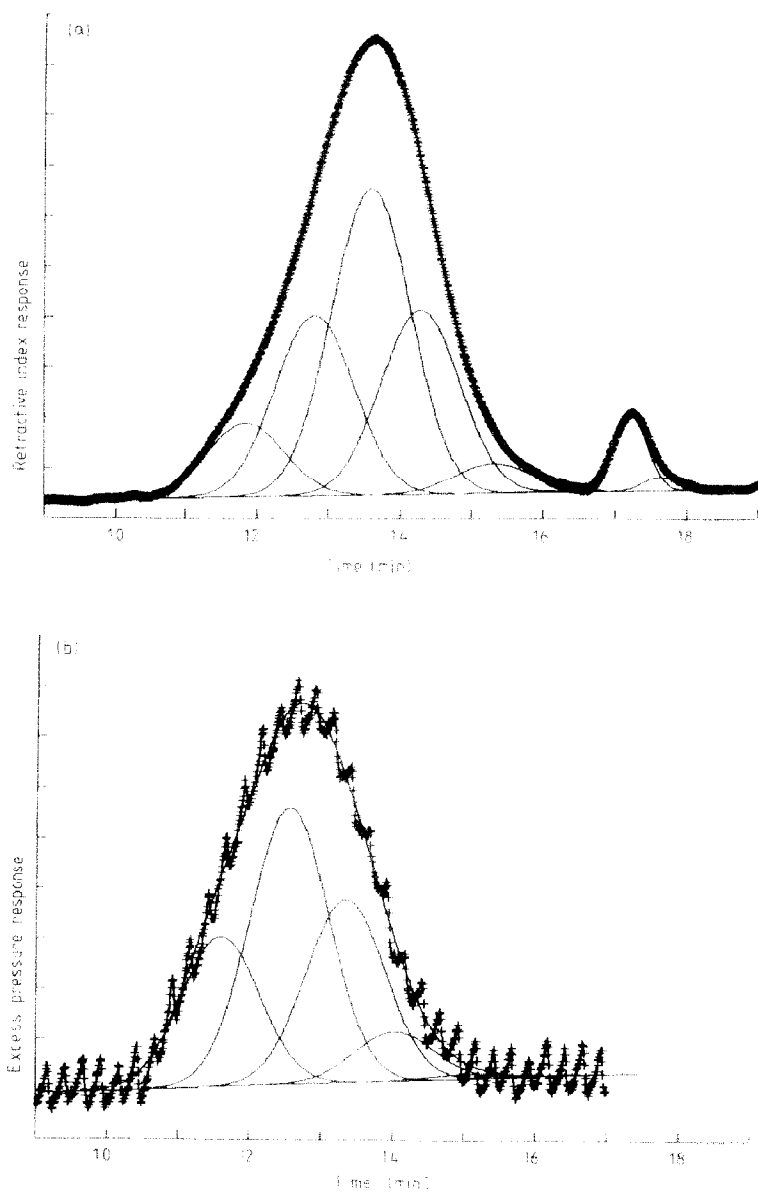
Fig. 4. Chromatograms of garlic skin pectin; injected concentration 2.58 mg mL -1 . For all other conditions see Fig. 2.
