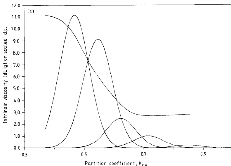
Fig. 5. Pomegranate pectin. (a) Superimposed curves of intrinsic viscosity (i.v.), differential refractive index (d.r.i.), and differential pressure (d.p.) as a function of K_{av} . Calculated from reconstructed chromatograms shown in Figs. 2a and 2b. (b) Intrinsic viscosity superimposed upon fitted components from d.r.i. (c) Intrinsic viscosity superimposed upon fitted components from d.p.
