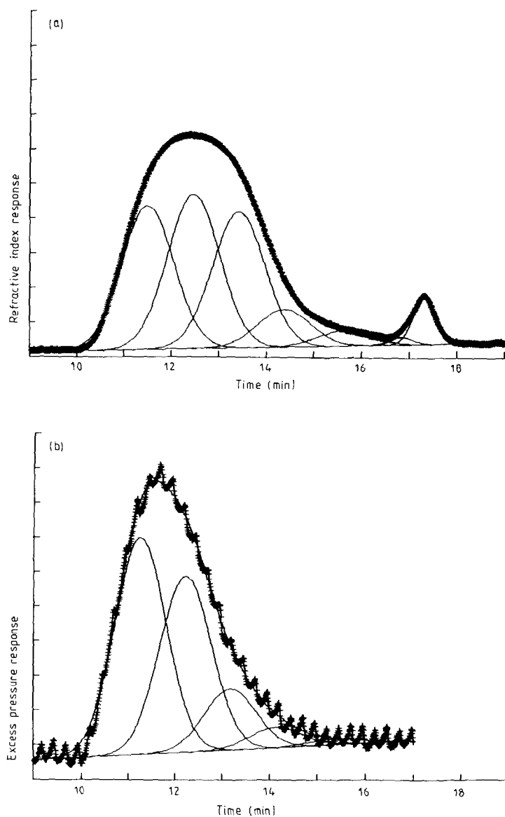
Fig. 3. Chromatograms of carrot pectin; injected concentration 2.60 mg/mL. For all other conditions see Fig. 2.
